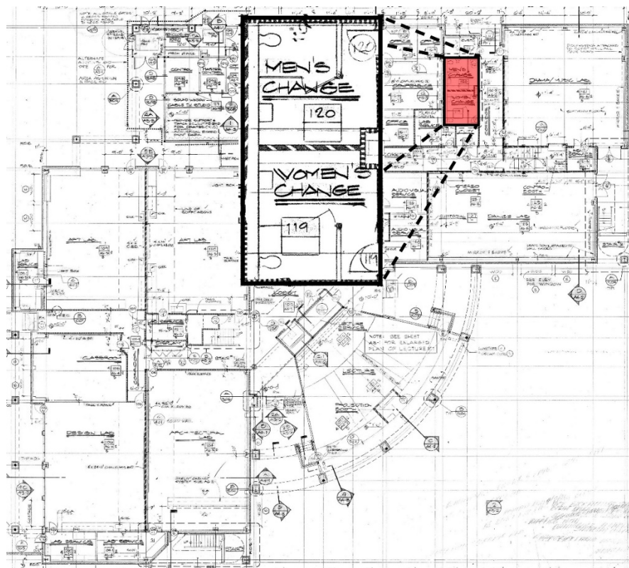
Building D Restroom Renovation (Single-User) at Santiago Canyon College Level One Floor Plan
