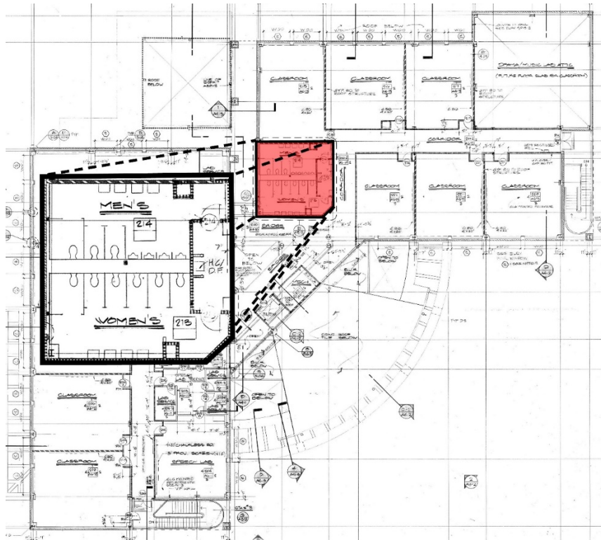
Building D Restroom Renovation (Multi-User) at Santiago Canyon College Level Two Floor Plan
