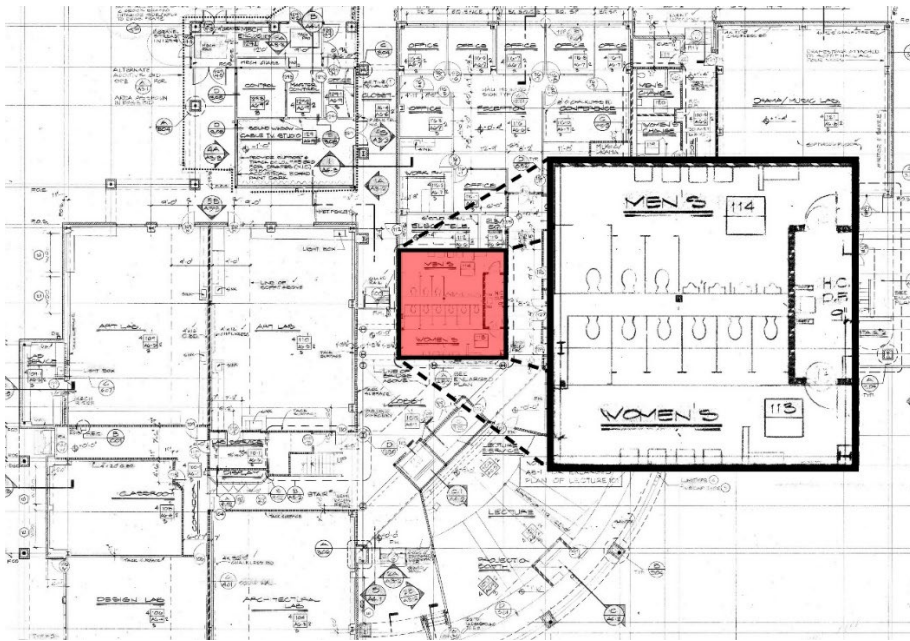
Building D Restroom Renovation (Multi-User) at Santiago Canyon College Level Two Floor Plan
